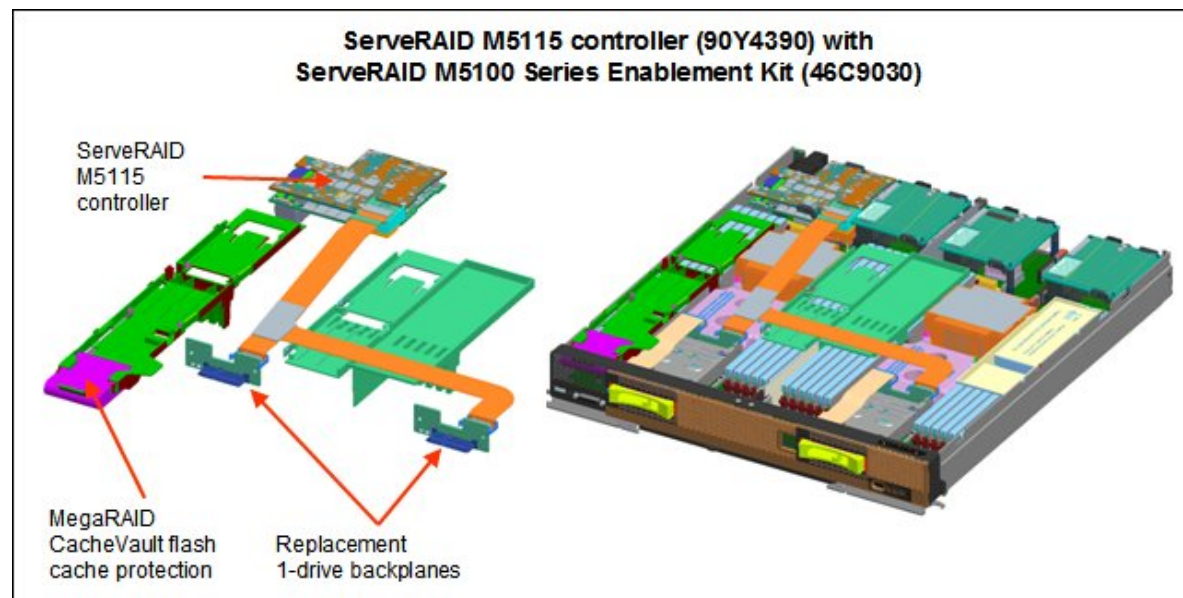
Figure 4. The ServerRAID M5115 and the Enablement Kit installed
