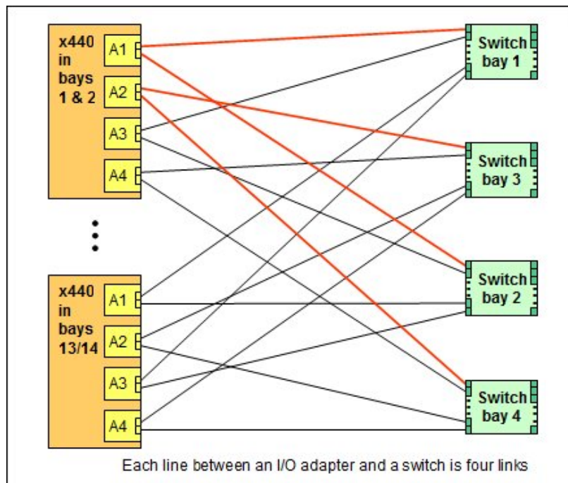
Figure 8. Logical layout of the
